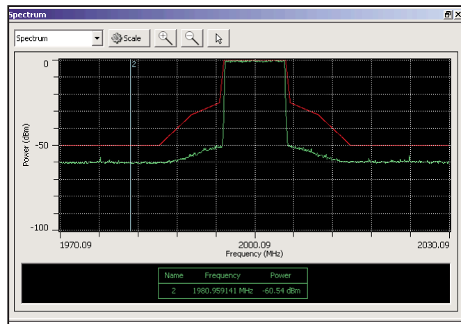
Figure 8. Spectral mask
