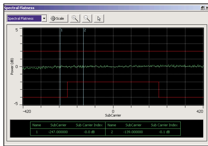
Figure 9. Spectral flatness
