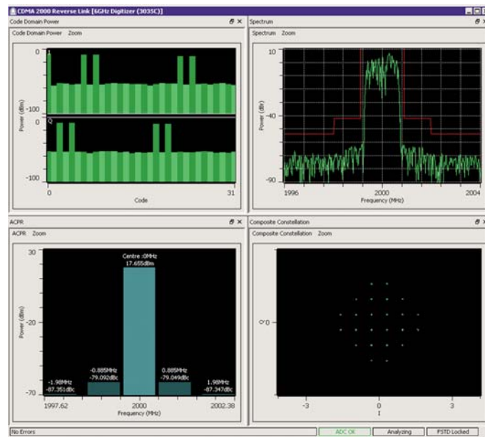
Figure 10. CDMA 2000 plug-in typical screenshot
