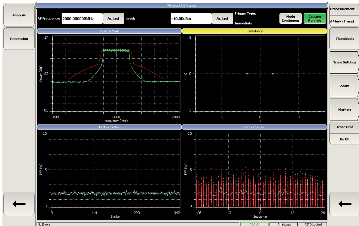
Figure 5. WLAN Measurements
