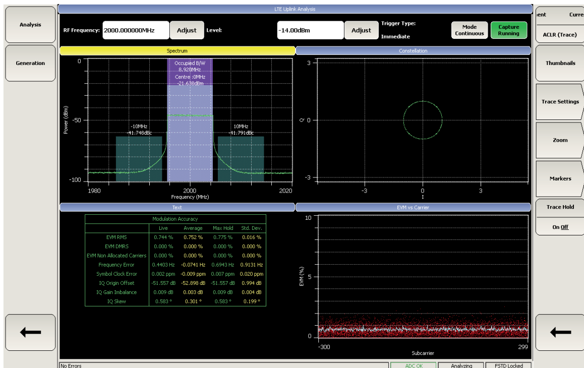
Figure 4. LTE FDD Measurements
