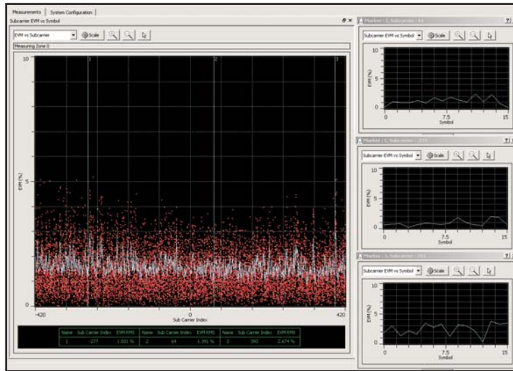
Figure 7. EVM Vs. Subcarrier with marker inspection
